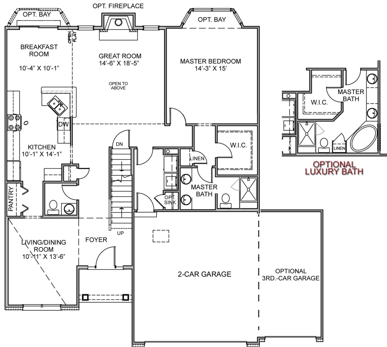
FIRST FLOOR
