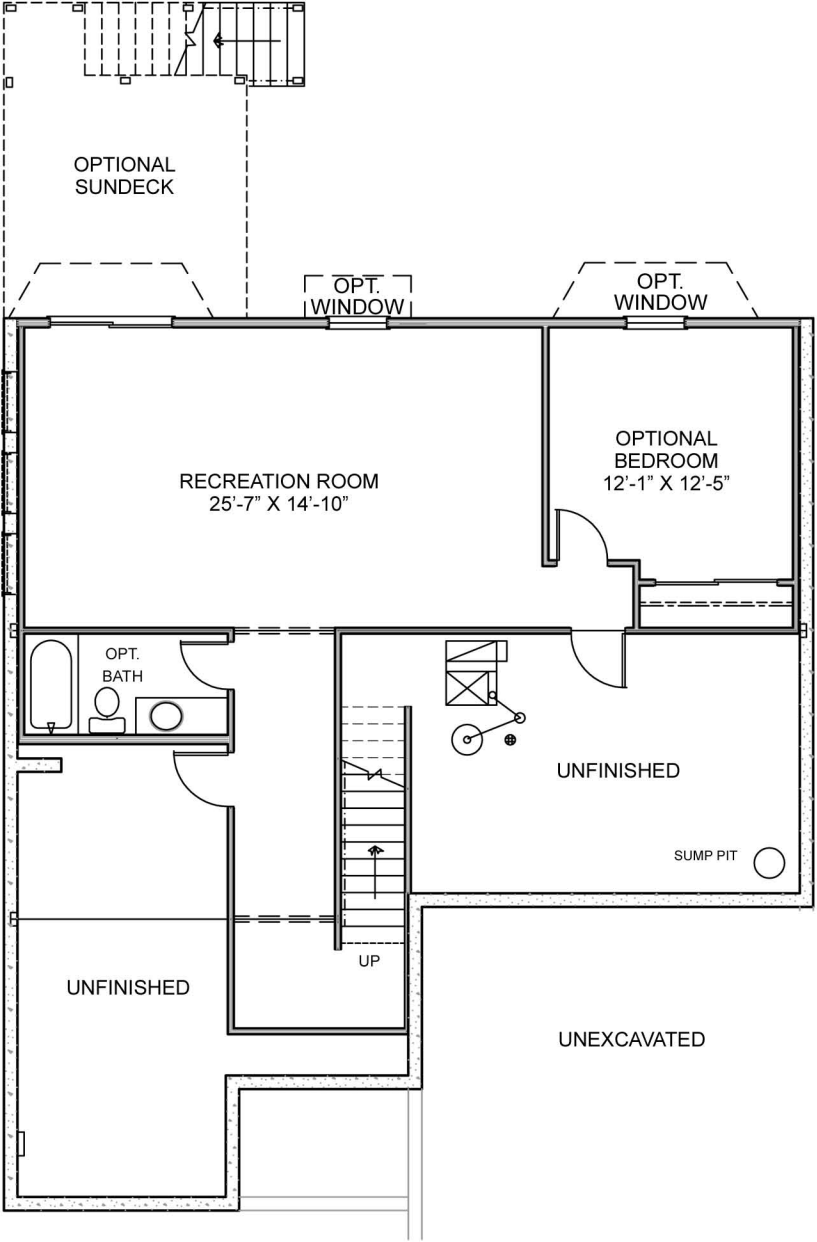
OPTIONAL FINISHED LOWER LEVEL
