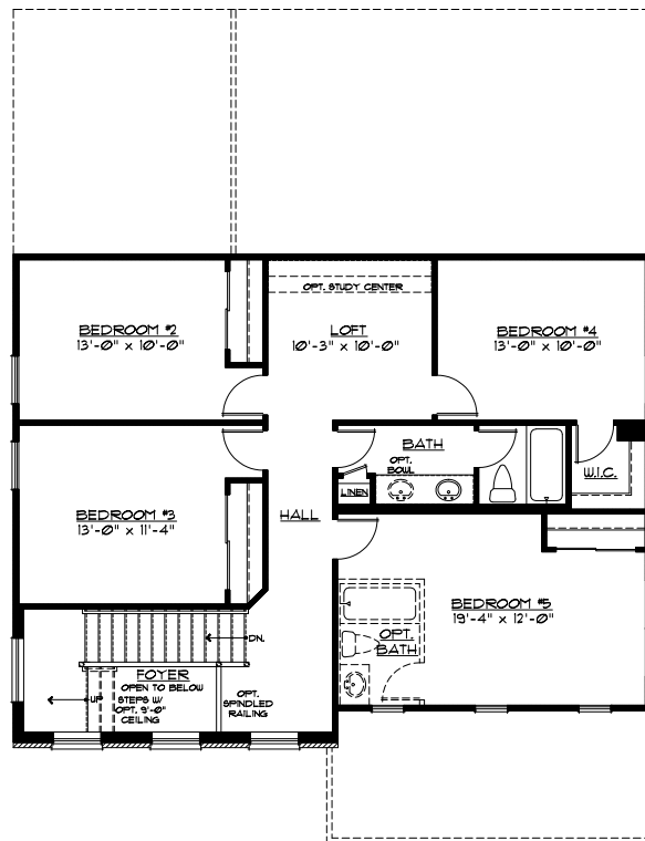
2ND FLOOR PLAN W/ OPT. BEDROOM #5
