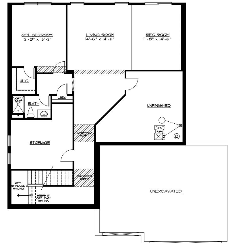
OPT. WALK OUT FINISHED LOWER LEVEL PLAN
