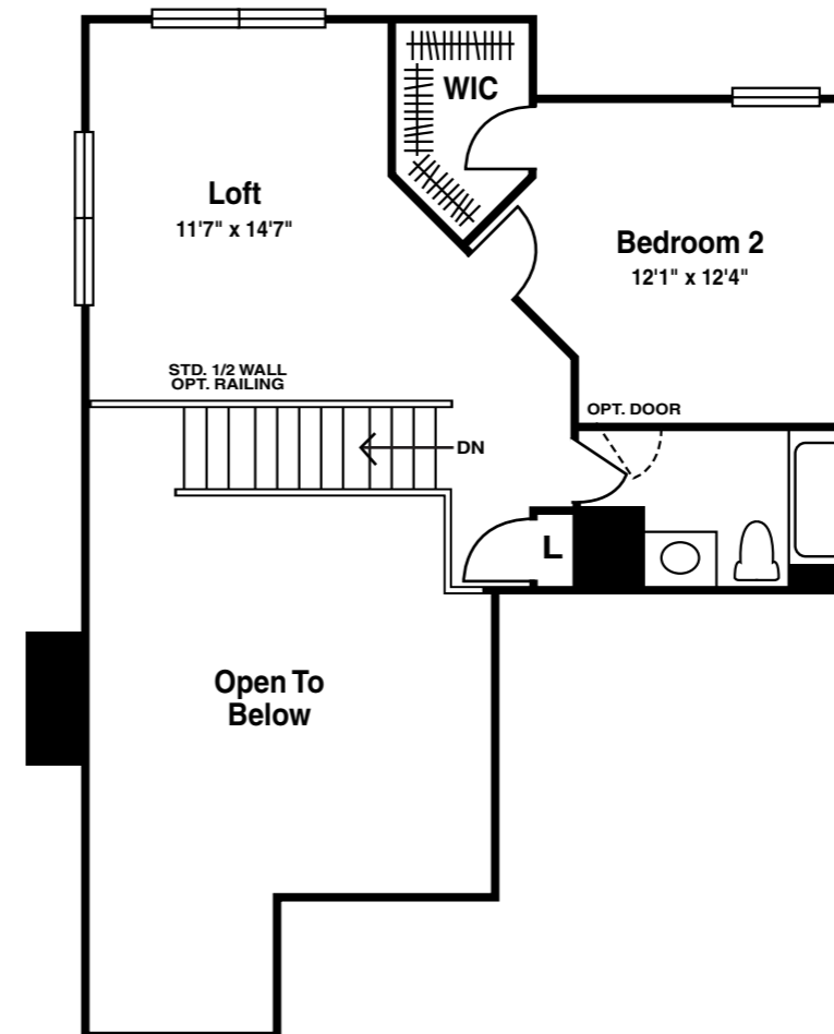
OPT. LOFT PLAN
